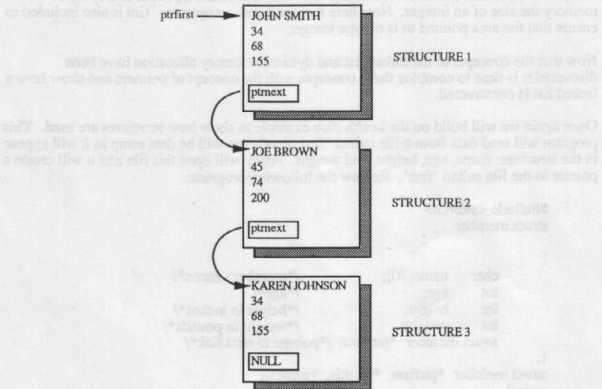
FIGURE 1. STRUCTURES FORMED INTO A LINKED LIST
